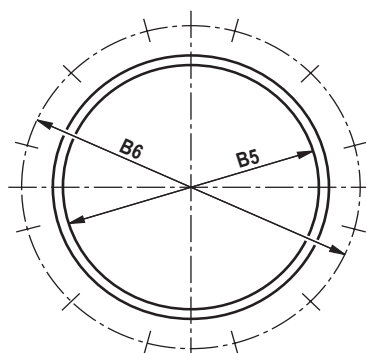
hole pattern
