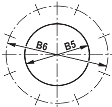
hole pattern
